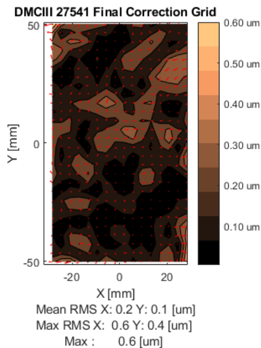
Figure 3: 2-D Image Residuals.
